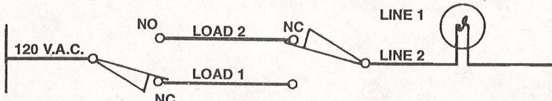
3-Way Switching
