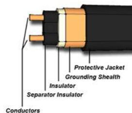
Heatizon Self Regulating Cable
