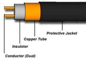
Heatizon Self Regulating Cable
