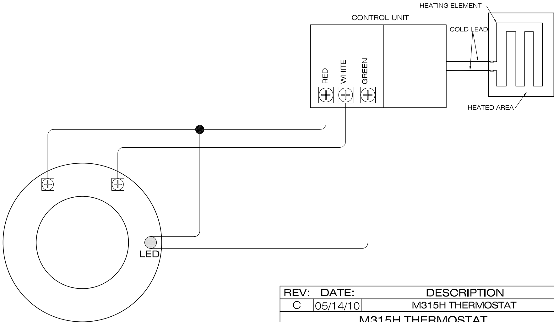
M315H THERMOSTAT
